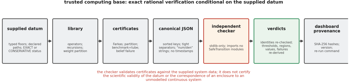
Figure 2: The certificate chain: the trusted computing base of an assessment verdict. Exact rational verification is conditional on the supplied datum; the checker validates certificates against the supplied system data and does not certify the datum’s scientific validity.
